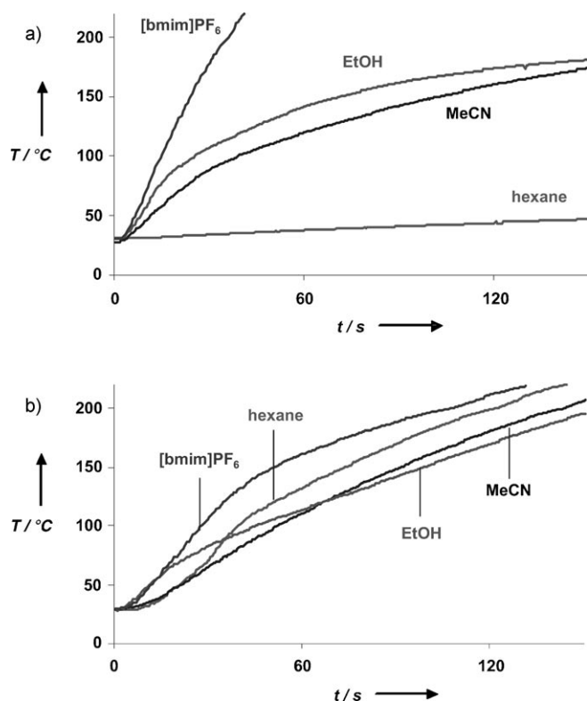
Figure 1. Heating rates for 3 mL samples of hexane ( \tan\delta=0.02 ), [3] MeCN ( \tan\delta=0.062 ), [3] EtOH ( \tan\delta=0.941 ), [3] and 1-butyl-3-methylimidazolium hexafluorophosphate ([bmim]PF 6 , \tan\delta>1 ) [8] at 130 W constant magnetron power in a 10 mL Pyrex vial (a), and in a custom-made SiC vial (b). Single-mode microwave irradiation, magnetic stirring, internal fiber-optic temperature measurement. [6]
